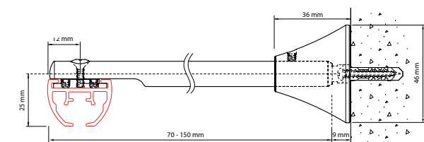
Wall mounting with adjustable extension bracket 6017
