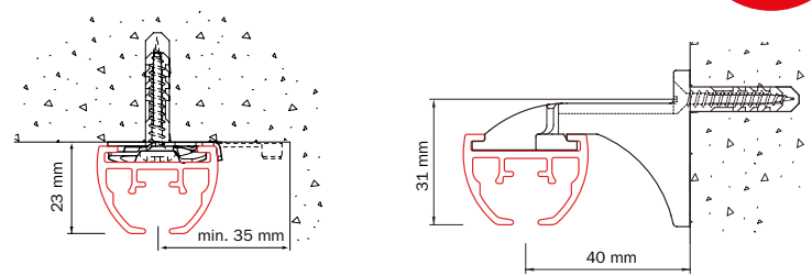
Ceiling mounting with ceiling mounting clamp 6050
