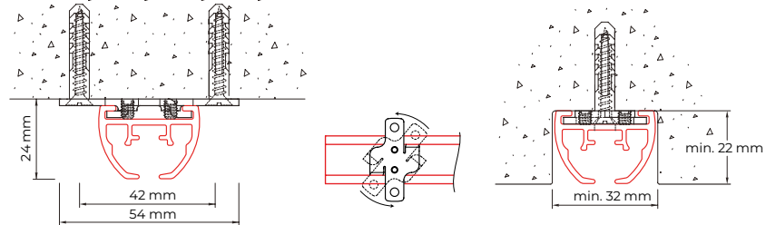
Ceiling mounting with bracket 6055-1000
