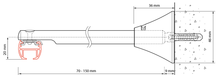
Wall mounting 4400 with adjustable extension bracket 4417
