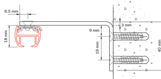
Wall mounting 4400 with spacer brackets 4415
