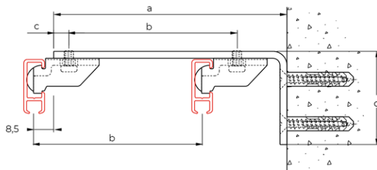
wall mounting with 2015 extension bracket and 2250 support
