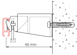
wall mounting using wall bracket 7451,
