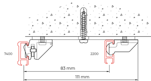
for perfect parallel mounting: use of double bracket 2216 with ceiling supports 7450 resp. 2250
